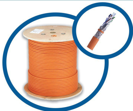
CAT6SF/UTP TEST FLUKE (CHANNEL)&(PERMANENT) INDOOR(PVC)&(LSZH) METERAGE:500
