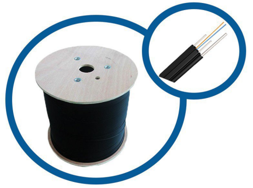
FTTH DROP OPTICAL FIBER CABLE (2CORE)(4CORE)(6CORE)(8CORE) SINGLE MODE (OUTDOOR/IN DOOR)(LSZH) METERAGE:1000
